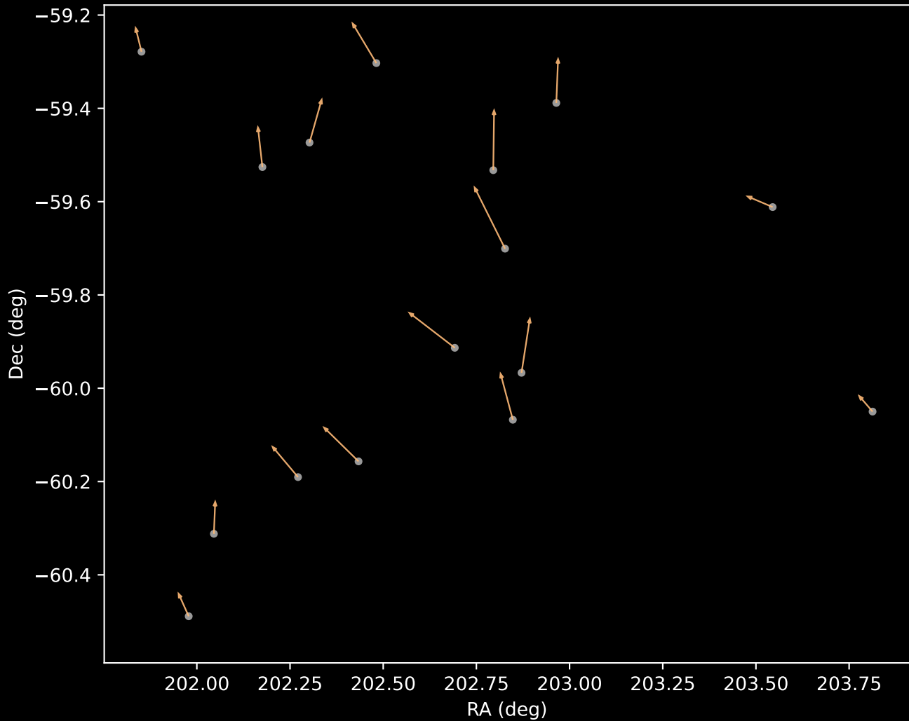
GALAH DR4 Cluster 3 Proper Motion Vectors (n=16)
