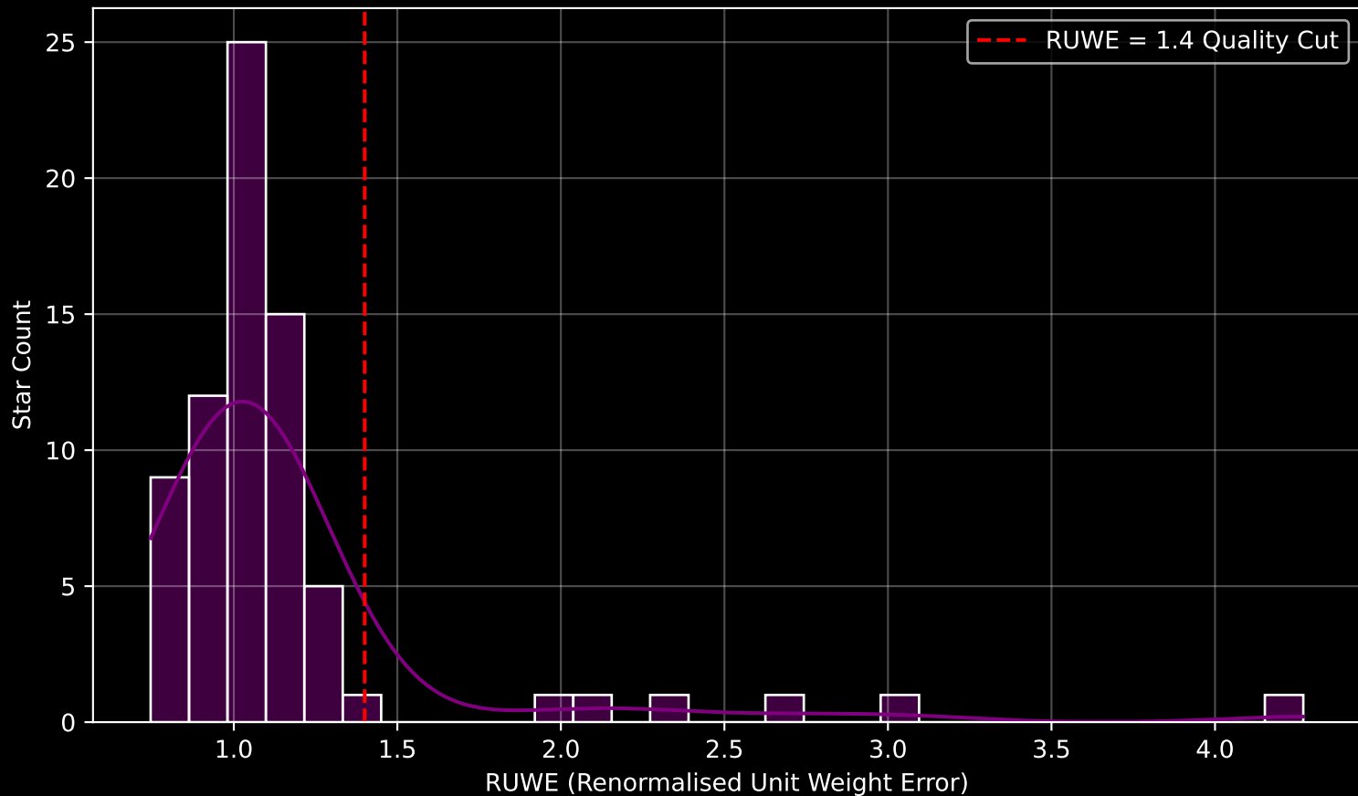
GALAH DR4 Field [7427] RUWE Distribution (n= 73)
