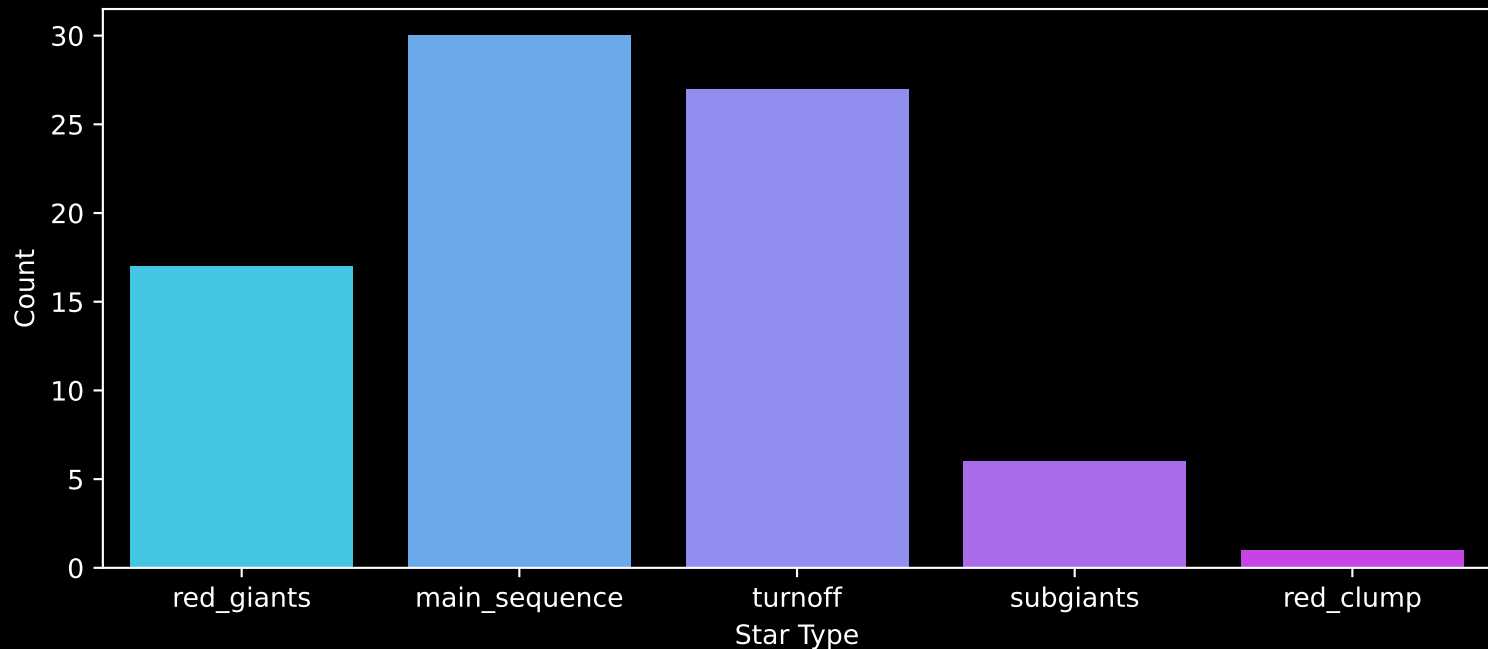
GALAH DR4 Field: [7427] Count plot of Star Type
