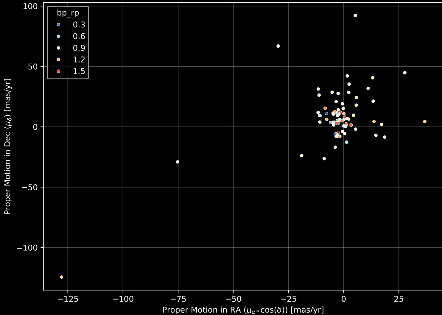
GALAH DR4 Field: [7427] Proper Motion Diagram (n= 81)
